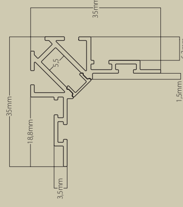
Star 62 Pladur esquina interior Internal corner plasterboard
