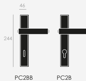
PLACA PC2 PC2 BACKPLATE
